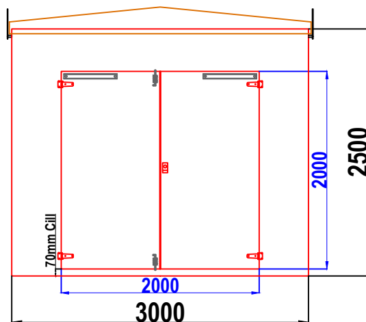
W10 WALK-IN GRP ENCLOSURE FRONT WALL ELEVATION WALL 1
