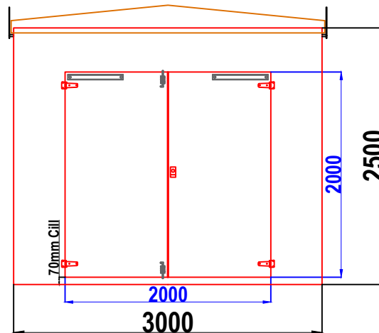
W11A WALK-IN GRP ENCLOSURE FRONT WALL ELEVATION WALL 1
