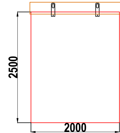
W11A WALK-IN GRP ENCLOSURE RIGHT HAND SIDE WALL ELEVATION WALL 3
