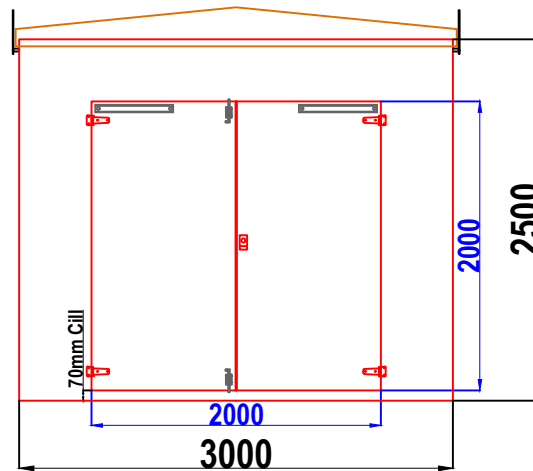
W12A WALK-IN GRP ENCLOSURE FRONT WALL ELEVATION WALL 1
