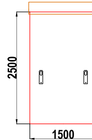
W8A WALK-IN GRP ENCLOSURE RIGHT HAND SIDE WALL ELEVATION WALL 3
