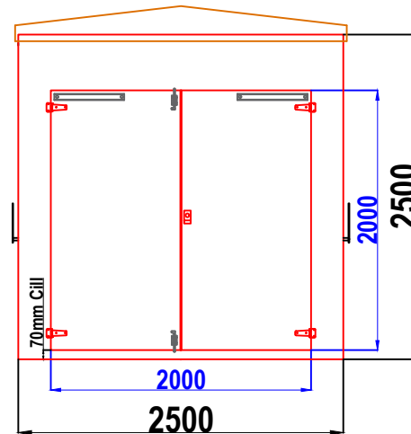
W8A WALK-IN GRP ENCLOSURE FRONT WALL ELEVATION WALL 1
