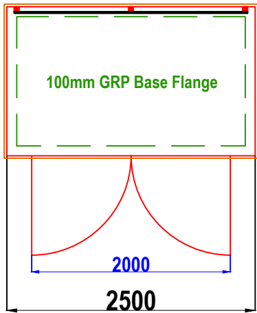
W8A WALK-IN GRP ENCLOSURE PLAN VIEW
