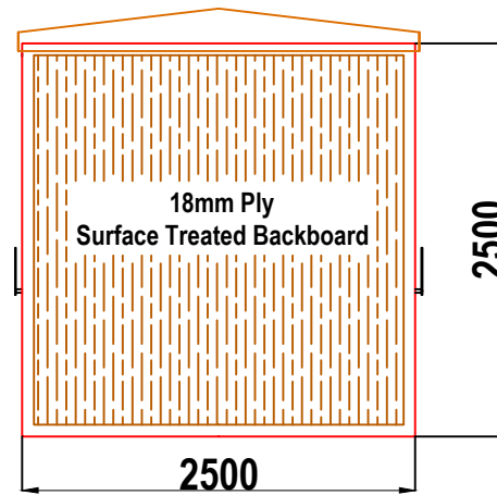
W8A WALK-IN GRP ENCLOSURE REAR WALL ELEVATION WALL 4
