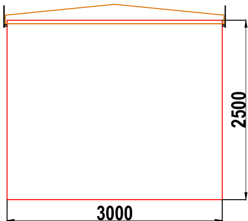
W9 WALK-IN GRP ENCLOSURE LEFT HAND SIDE WALL ELEVATION WALL 2
