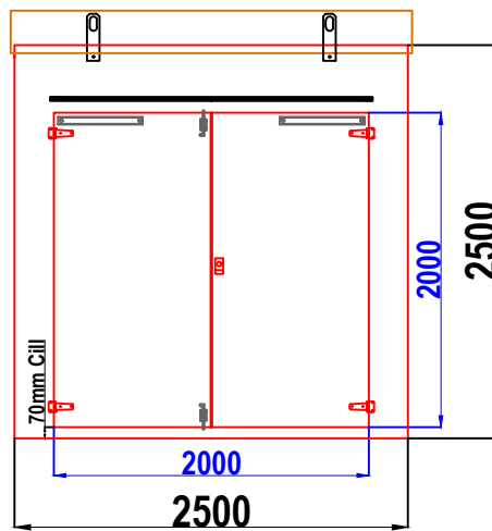
W9 WALK-IN GRP ENCLOSURE FRONT WALL ELEVATION WALL 1
