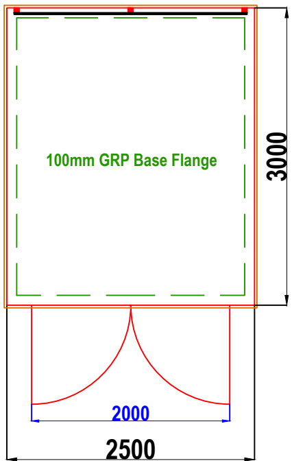
W9 WALK-IN GRP ENCLOSURE PLAN VIEW
