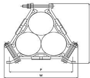
Two Bolt
