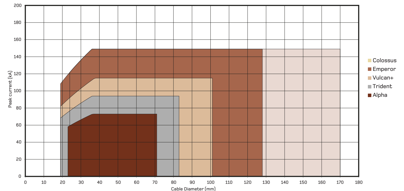
ELLIS CLEAT RANGE. CLEATS SPACED AT 600MM
