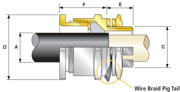
Wire Braid Pig Tail
