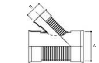
Ridgidrain 45° junctions All junctions are triple socketed. Order seals and couplings separately.
