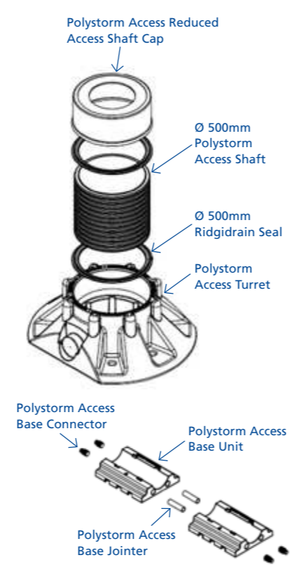
Please note: The Polystorm Access turret and base assembly are black. They are shown blue for illustration purposes.
