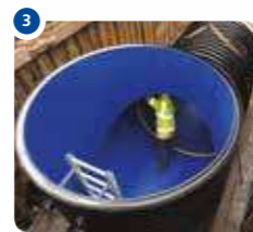
Ridgistorm-XL An engineered, large diameter pipe solution for surface water, foul water and combined sewer applications.
