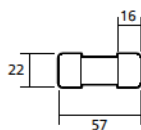
Fuselink to BS HD 60259-3 2010* for use with 60A/80A carrier
