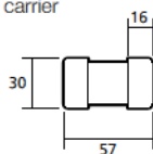
Fuselink to BS HD 60259-3 2010* for use with 100A carrier
