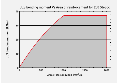
200mm STEPOC
