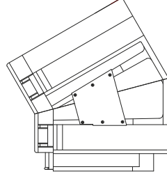
SIZE 430 - Gradient Trough (up) (GT-430-05)
