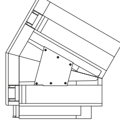
SIZE 430 - Gradient Trough (down) (GT-430-06)
