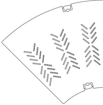
SIZE 430 - Straight Trough (GT-430-02)
