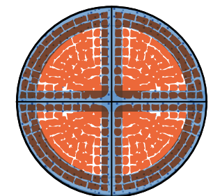
Figure 2: AC current flows on Milliken conductor.
