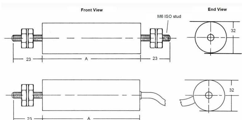
Figure 1 - Design and Dimensions (mm) for Standard Format and Flying Lead SVL Surge Diverters
