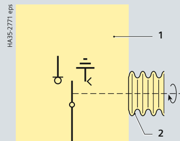
Three-position disconnecter
