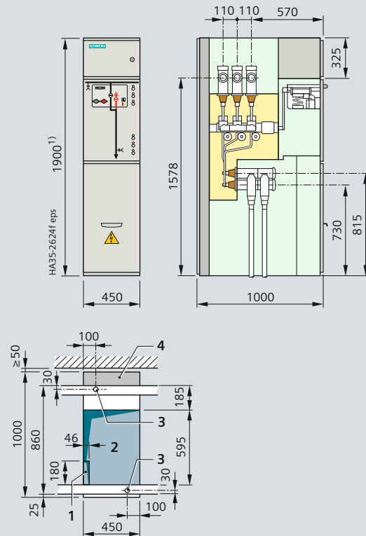
Disconnecter panel
