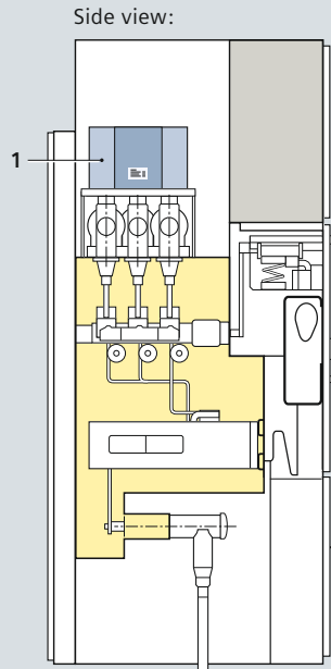
1 Busbar voltage transformer
