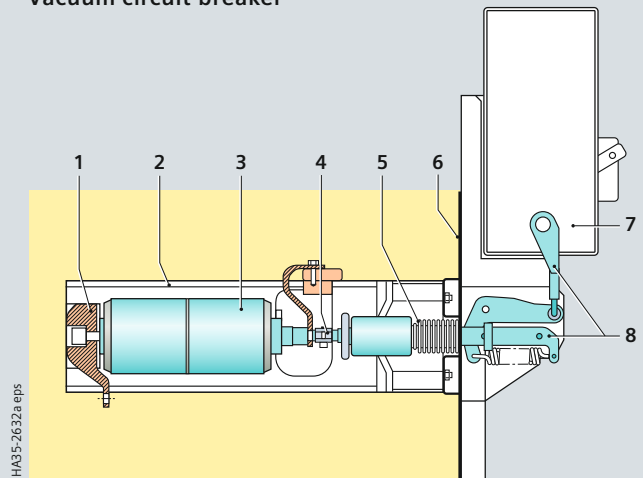
Section through the vacuum circuit-breaker
