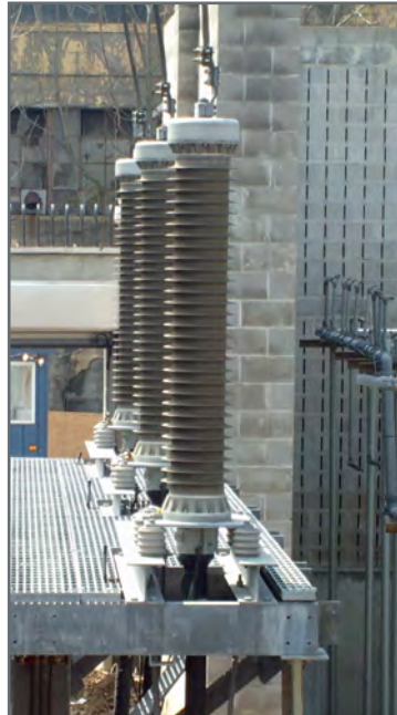
▲ Outdoor termination
