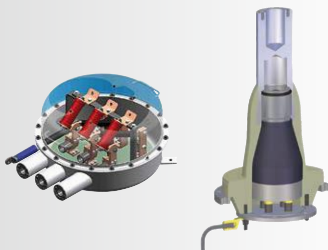
Link box with voltage limiters and dead-end plug for KSEV/KTEV
