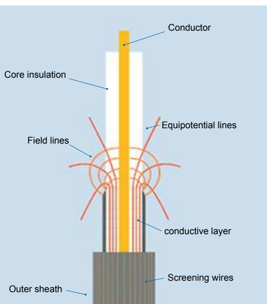
Electrical field without stress control (figure 1)
