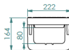
MMtrough cross-section detail
