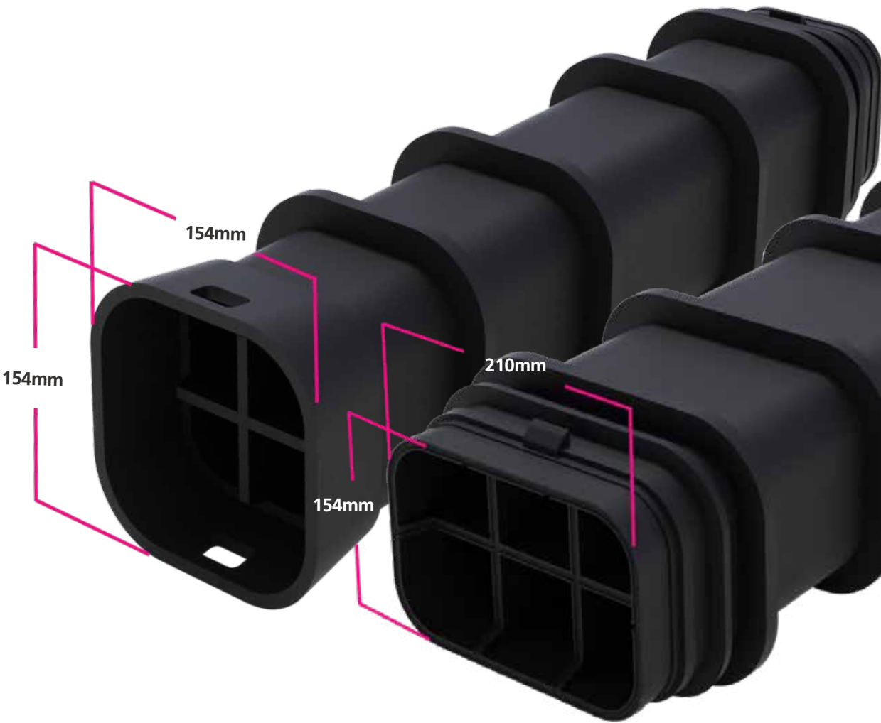
Duct face and inner ducts can be sealed to enhance cable blowing capabilities
