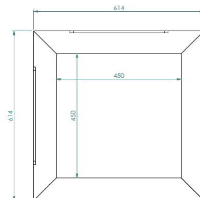
RapidSTACK™ cross-section top view
