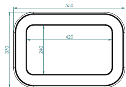
ULTIMA cross-section top view
