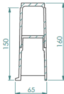
ULTIMA cross-section detail
