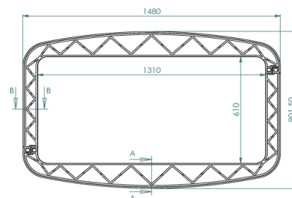
Fortress cross-section top view
