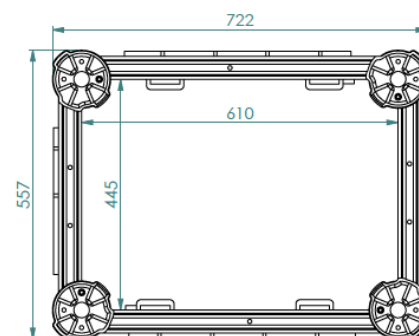
Fortress cross-section top view
