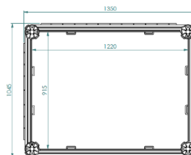
Fortress cross-section top view
