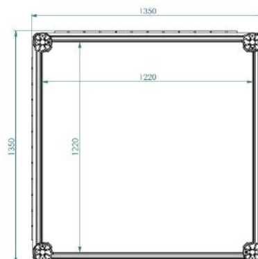
Fortress cross-section top view
