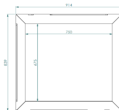
RapidSTACK™ cross-section top view
