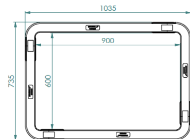
ULTIMA Connect cross-section top view
