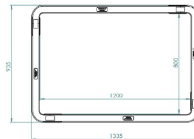
ULTIMA Connect cross-section top view
