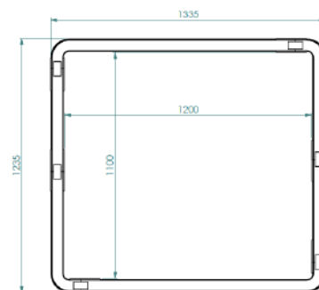
ULTIMA Connect cross-section top view
