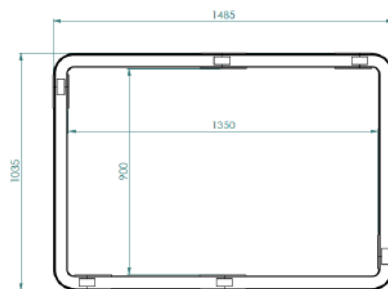
ULTIMA Connect cross-section top view
