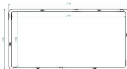
ULTIMA Connect cross-section top view
