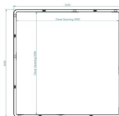
ULTIMA Connect cross-section top view
