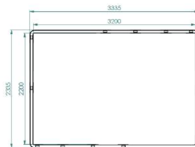
ULTIMA Connect cross-section top view
