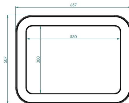
ULTIMA cross-section top view
