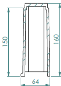
ULTIMA cross-section detail
