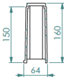
ULTIMA cross-section detail
