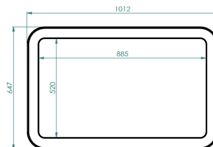
ULTIMA cross-section top view
