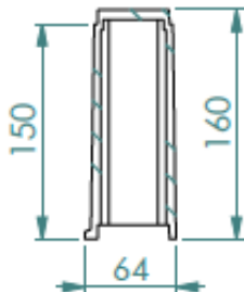
ULTIMA cross-section detail
