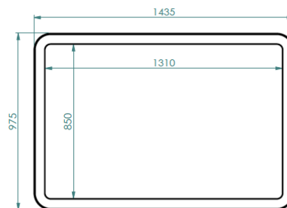
ULTIMA cross-section top view
