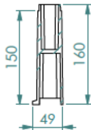
ULTIMA cross-section detail
