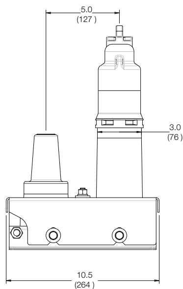
Clēer Loadbreak Connector Assembly (Square SS Bracket).
