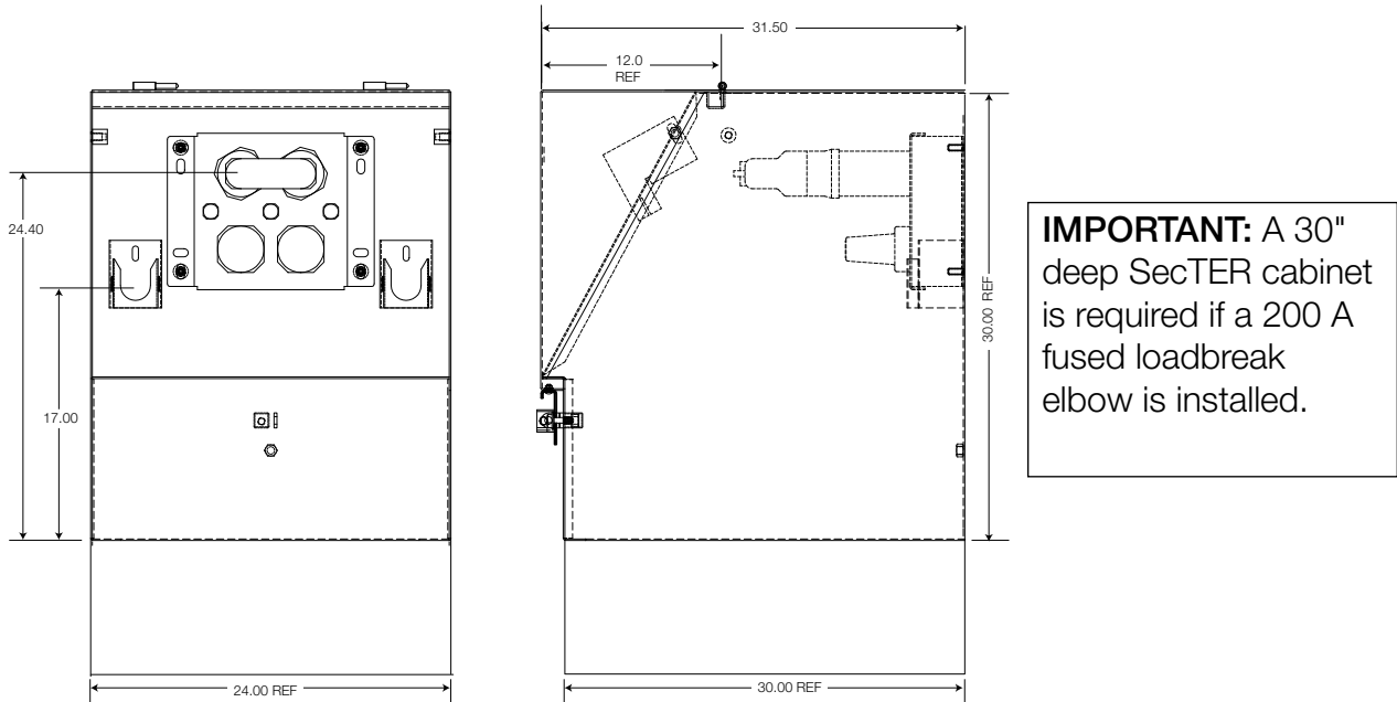
Single-phase SecTER Cabinet, Catalog Number SEC1P__CLEERA2DP.
