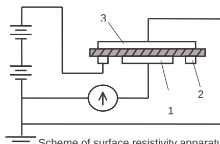
Scheme of surface resistivity apparatus
