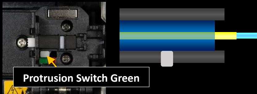
Protrusion Switch
