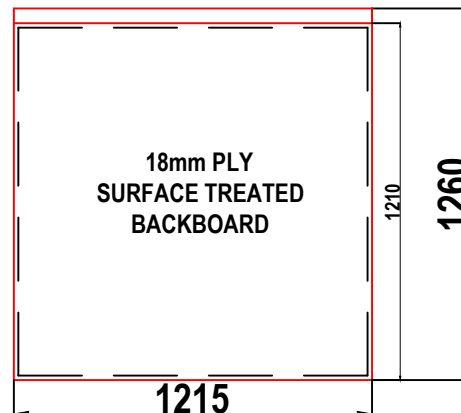
D2 GRP CABINET REAR WALL ELEVATION WALL 4
