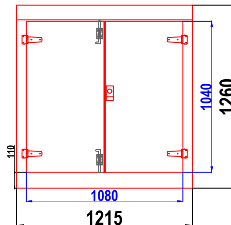
D2 GRP CABINET FRONT WALL ELEVATION WALL 1
