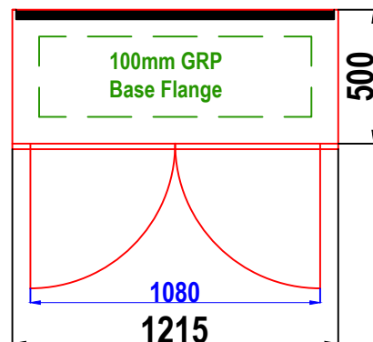
D2 GRP CABINET PLAN VIEW
