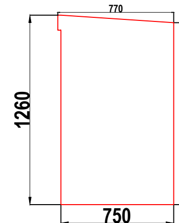
D2A GRP CABINET RIGHT HAND SIDE WALL ELEVATION WALL 3
