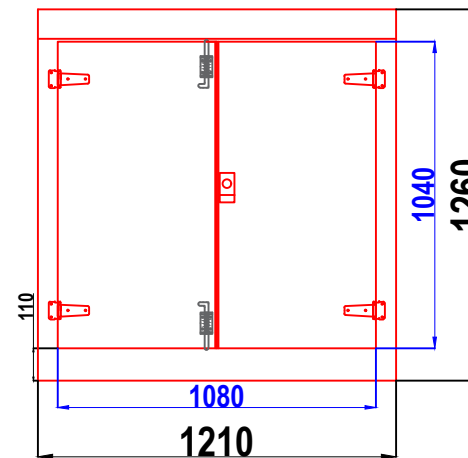
D2A GRP CABINET FRONT WALL ELEVATION WALL 1
