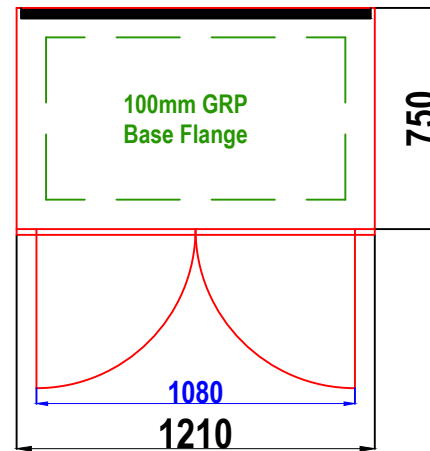
D2A GRP CABINET PLAN VIEW
