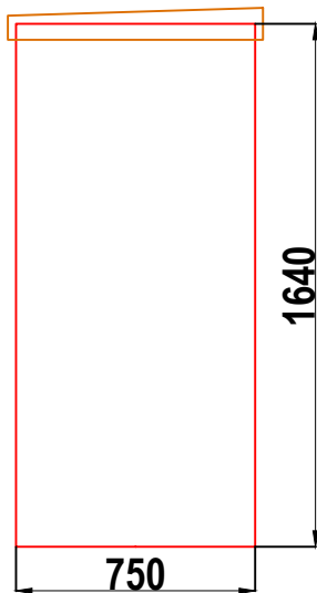
D4 GRP CABINET LEFT HAND SIDE WALL ELEVATION WALL 2
