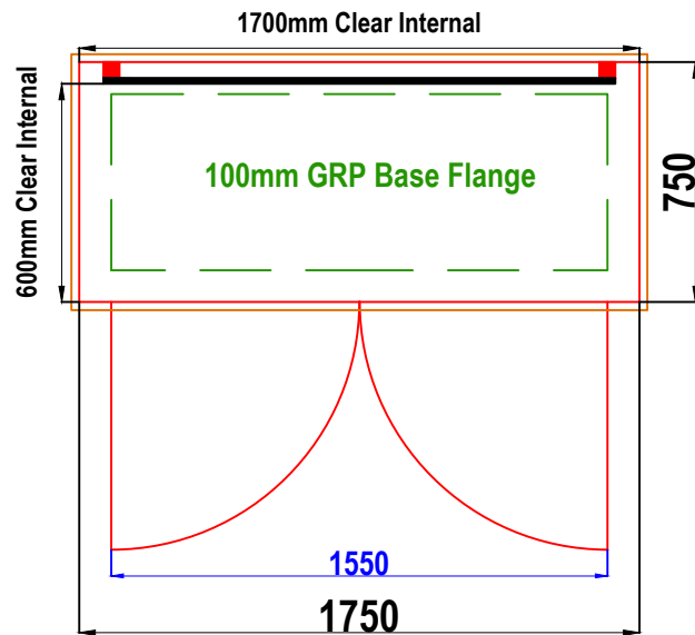
D4 GRP CABINET PLAN VIEW
