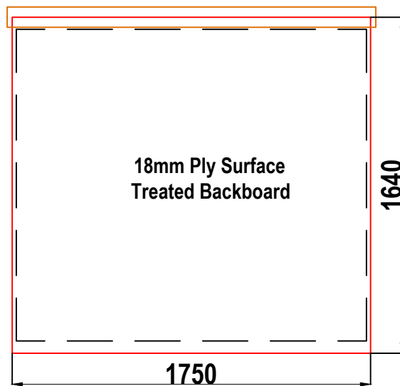
D4 GRP CABINET REAR WALL ELEVATION WALL 4
