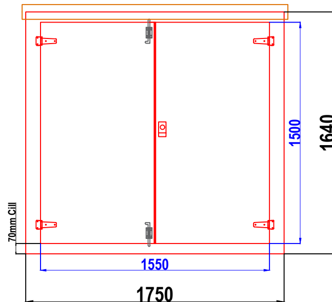
D4 GRP CABINET FRONT WALL ELEVATION WALL 1
