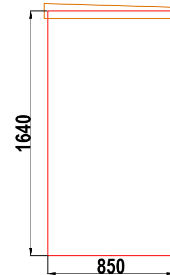
D5 GRP CABINET RIGHT HAND SIDE WALL ELEVATION WALL 3
