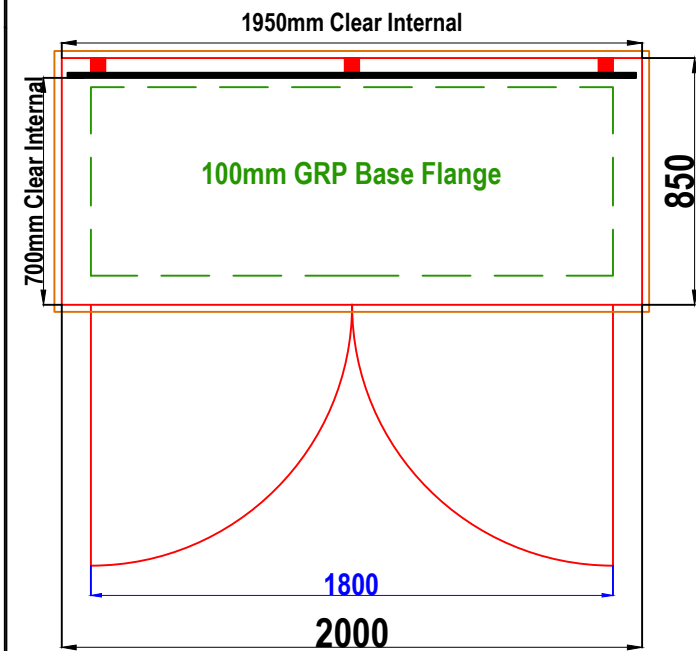
D5 GRP CABINET PLAN VIEW
