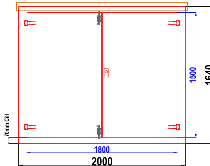
D5 GRP CABINET FRONT WALL ELEVATION WALL 1
