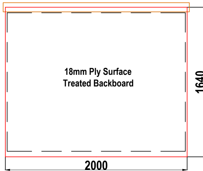
D5 GRP CABINET REAR WALL ELEVATION WALL 4
