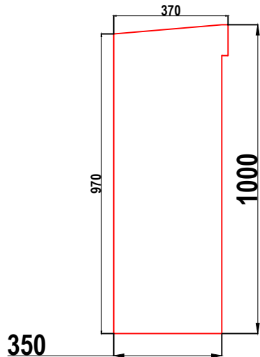
S2 GRP CABINET LEFT HAND SIDE WALL ELEVATION WALL 2
