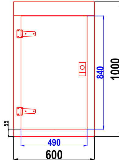
S2 GRP CABINET FRONT WALL ELEVATION WALL 1
