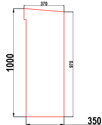
S2 GRP CABINET RIGHT HAND SIDE WALL ELEVATION WALL 3
