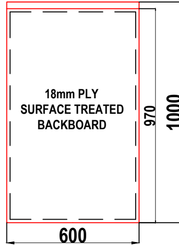
S2 GRP CABINET REAR WALL ELEVATION WALL 4
