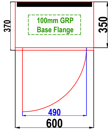
S2 GRP CABINET PLAN VIEW
