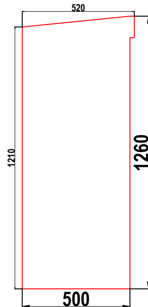
S5 GRP CABINET LEFT HAND SIDE WALL ELEVATION WALL 2
