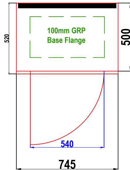
S5 GRP CABINET PLAN VIEW
