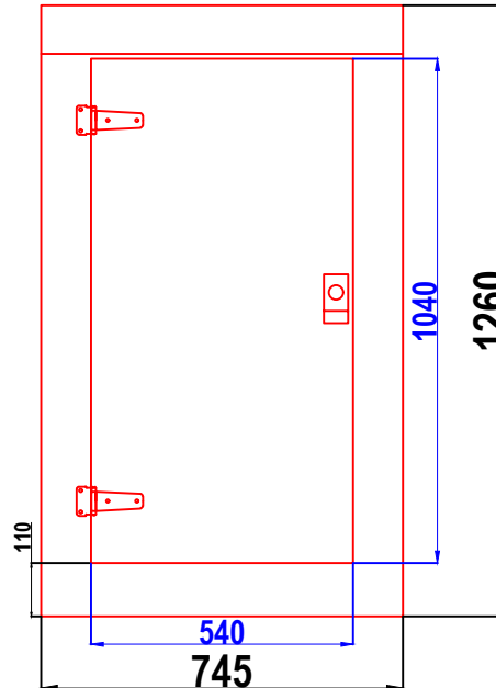
S5 GRP CABINET FRONT WALL ELEVATION WALL 1
