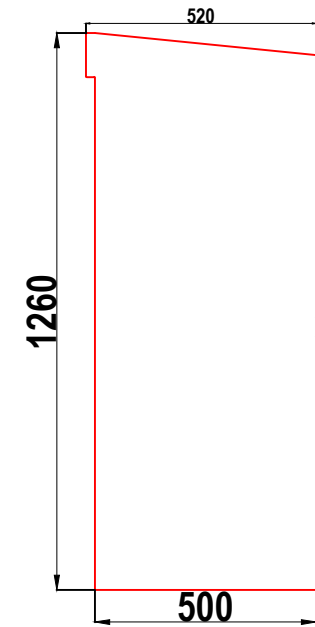
S5 GRP CABINET RIGHT HAND SIDE WALL ELEVATION WALL 3
