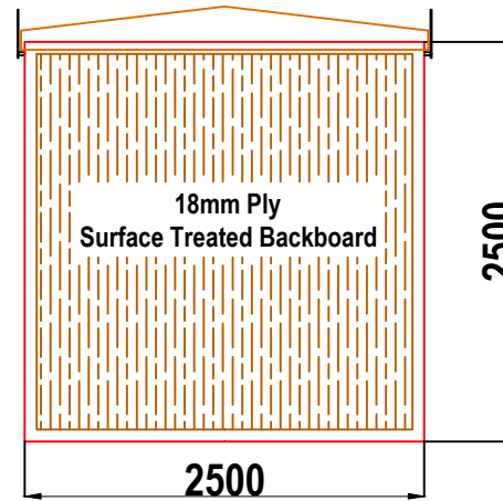
W5 WALK-IN GRP ENCLOSURE REAR WALL ELEVATION WALL 4
