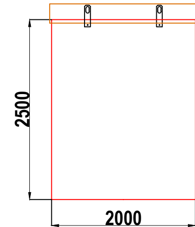
W5 WALK-IN GRP ENCLOSURE RIGHT HAND SIDE WALL ELEVATION WALL 3
