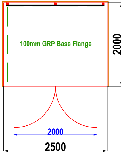
W5 WALK-IN GRP ENCLOSURE PLAN VIEW
