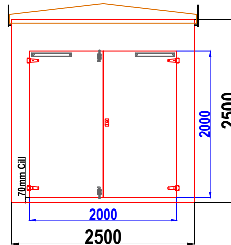
W5 WALK-IN GRP ENCLOSURE FRONT WALL ELEVATION WALL 1
