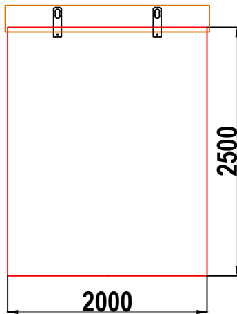
W5 WALK-IN GRP ENCLOSURE LEFT HAND SIDE WALL ELEVATION WALL 2
