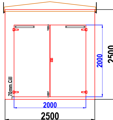
W5A WALK-IN GRP ENCLOSURE FRONT WALL ELEVATION WALL 1
