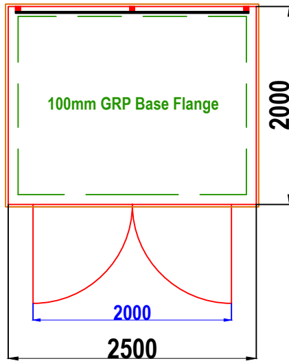
W5A WALK-IN GRP ENCLOSURE PLAN VIEW
