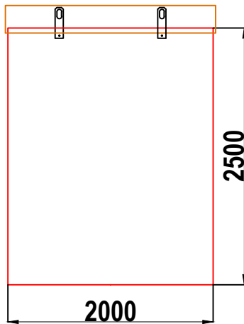
W5A WALK-IN GRP ENCLOSURE LEFT HAND SIDE WALL ELEVATION WALL 2
