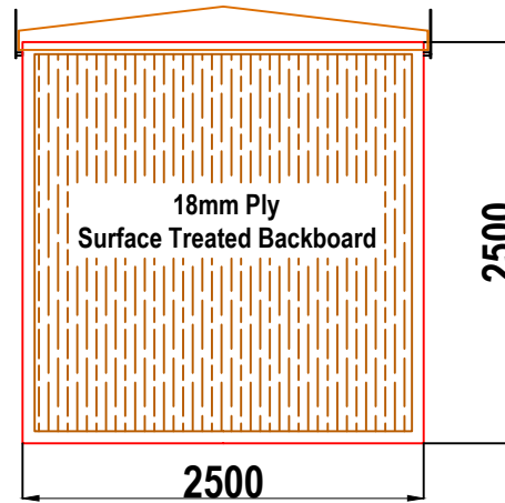
W5A WALK-IN GRP ENCLOSURE REAR WALL ELEVATION WALL 4
