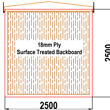
W6 WALK-IN GRP ENCLOSURE REAR WALL ELEVATION WALL 4
