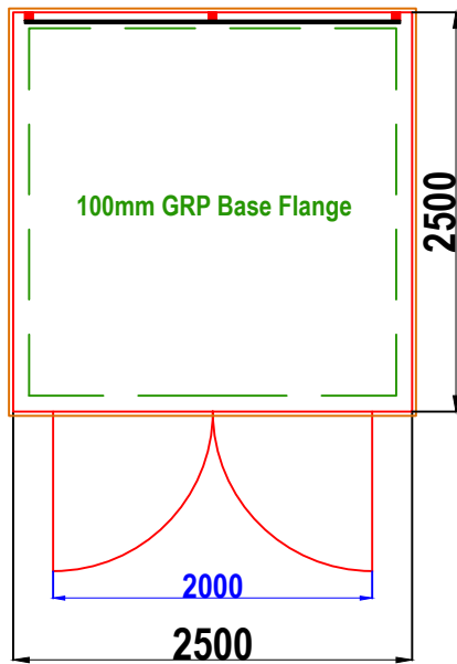
W6 WALK-IN GRP ENCLOSURE PLAN VIEW
