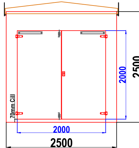
W6 WALK-IN GRP ENCLOSURE FRONT WALL ELEVATION WALL 1
